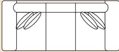
1500 Sofa Overall: H 36 W 102 D 43 Seating: H 16 W 76 D 24 Seat Height: 20 Arm Height: 27 Pillows: 2 P23, 2 P21
