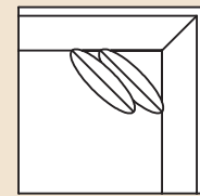
1561 Corner Chair Overall: H 36 W 43 D 43 Seating: H 16 W 24 D 24 Seat Height: 20 Arm Height: 27 Pillows: 1 P23, 1 P21
