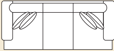
6000 Sofa Overall: H 38 W 97 D 42 Seating: H 18 W 78 D 26 Seat Height: 20 Arm Height: 25 Pillows: 4 P23
