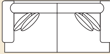
6075 Sofa Overall: H 38 W 89 D 42 Seating: H 18 W 70 D 26 Seat Height: 20 Arm Height: 25 Pillows: 4 P23
