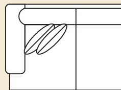
6072 LAF One Arm Loveseat 6073 RAF One Arm Loveseat Overall: H 38 W 59 D 42 Seating: H 18 W 50 D 26 Seat Height: 20 Arm Height: 25 Pillows: 2 P23
