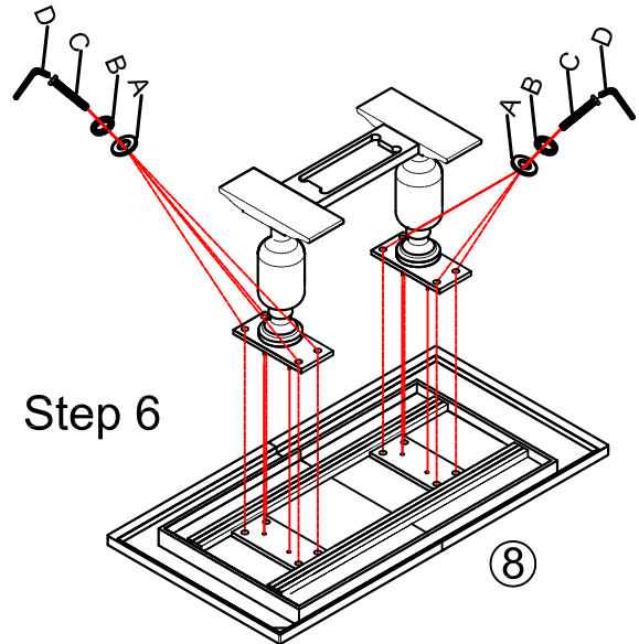
Step 6: Attach complete base to top panel (8).
