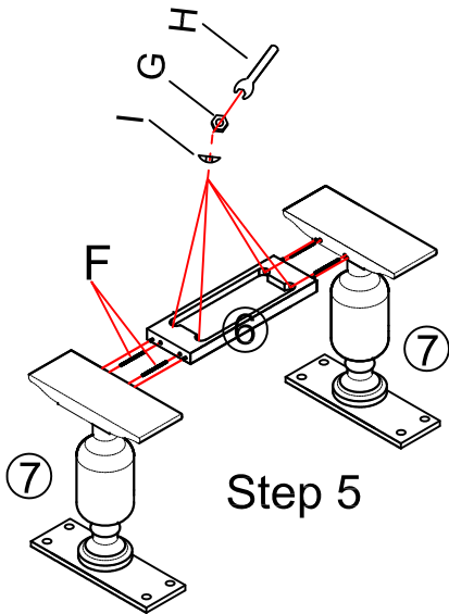
Step 5: Attach bottom stretcher (6) between short pedestals (7).
